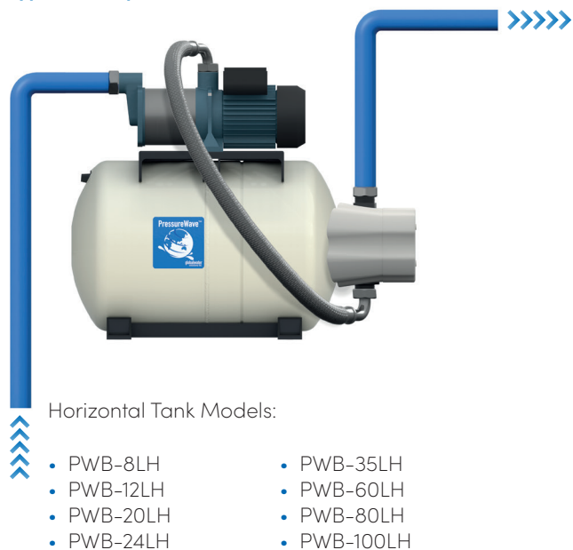
Typical PumpWave™ 2 Installation
